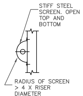
TRASH SCREEN DETAIL
