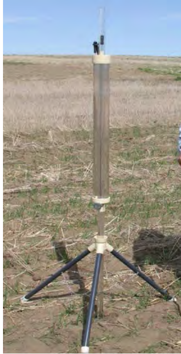
Figure C-3: Guelph Permeameter for Shallow Borehole Permeability
