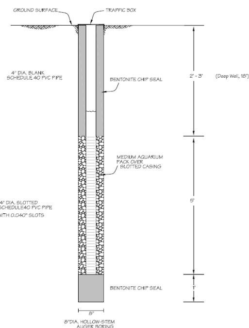
Figure C-4: Falling-Head Permeameter for Deep Borehole Permeability
