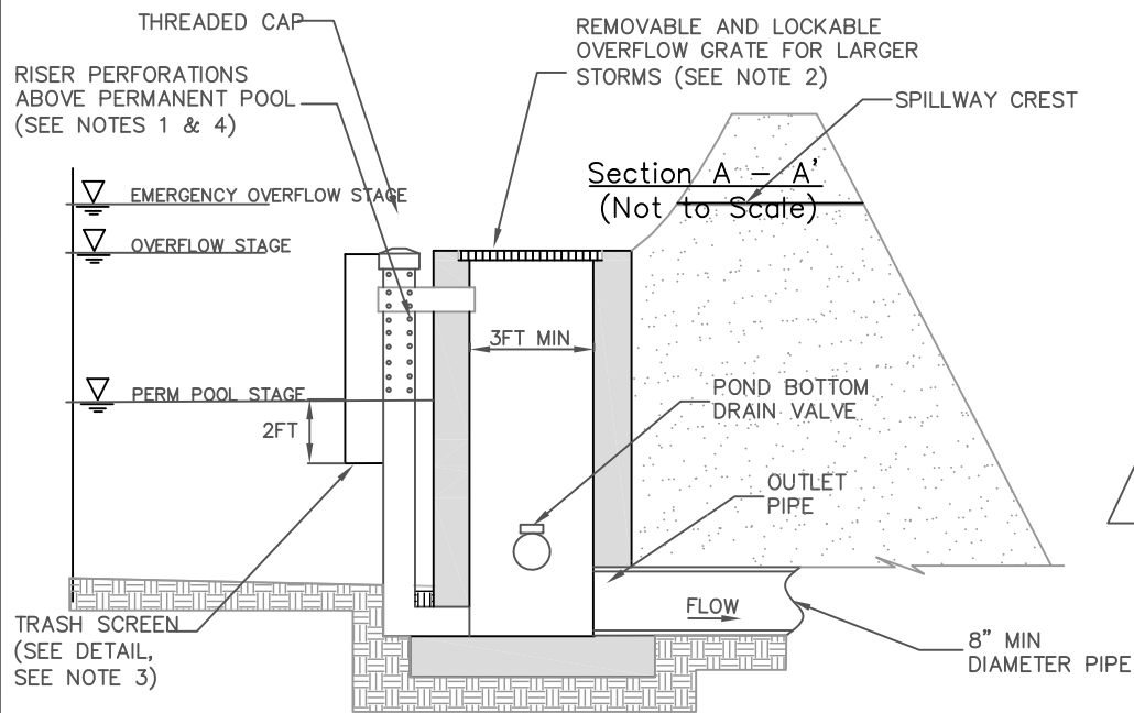
Perforated Riser Outlet Structure (Not to Scale)
