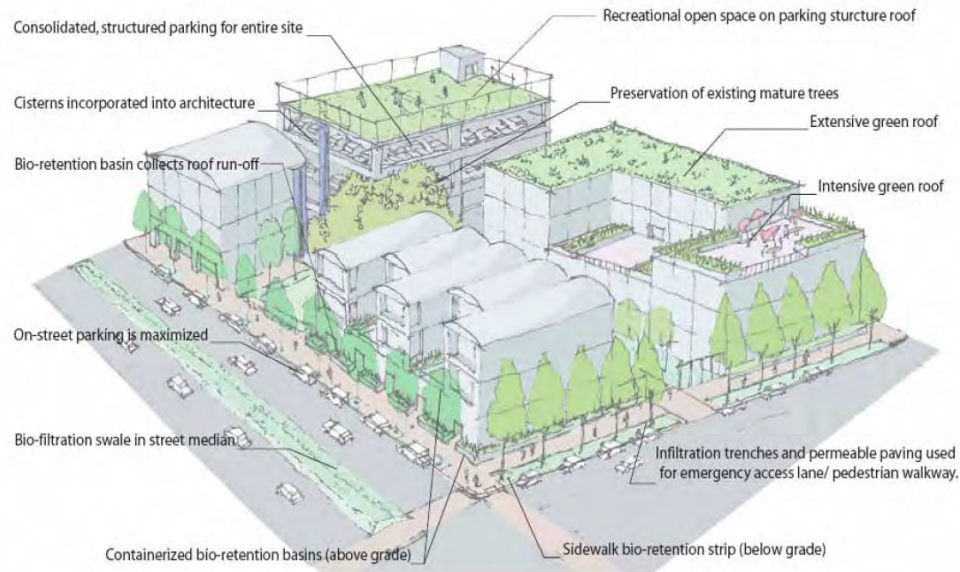
LID BMPs Considered at Various Scales
