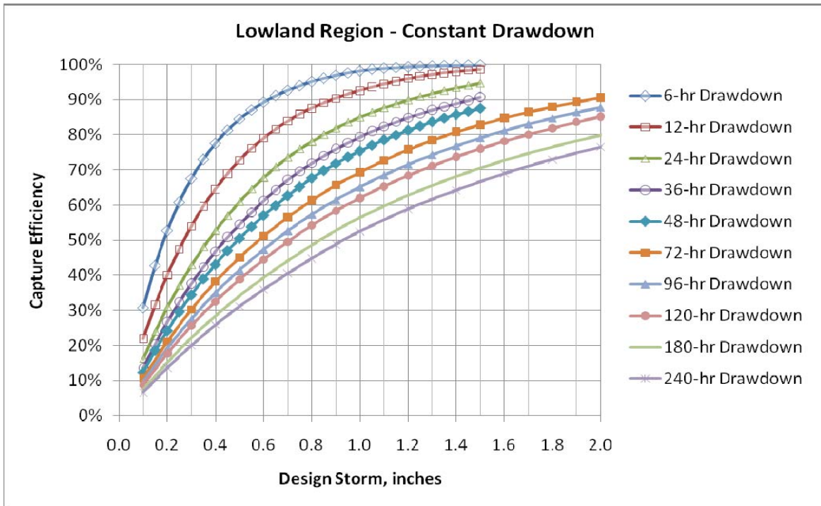
Figure D-1: Percent capture nomograph for systems with constant drawdown lowland regions of Ventura County
