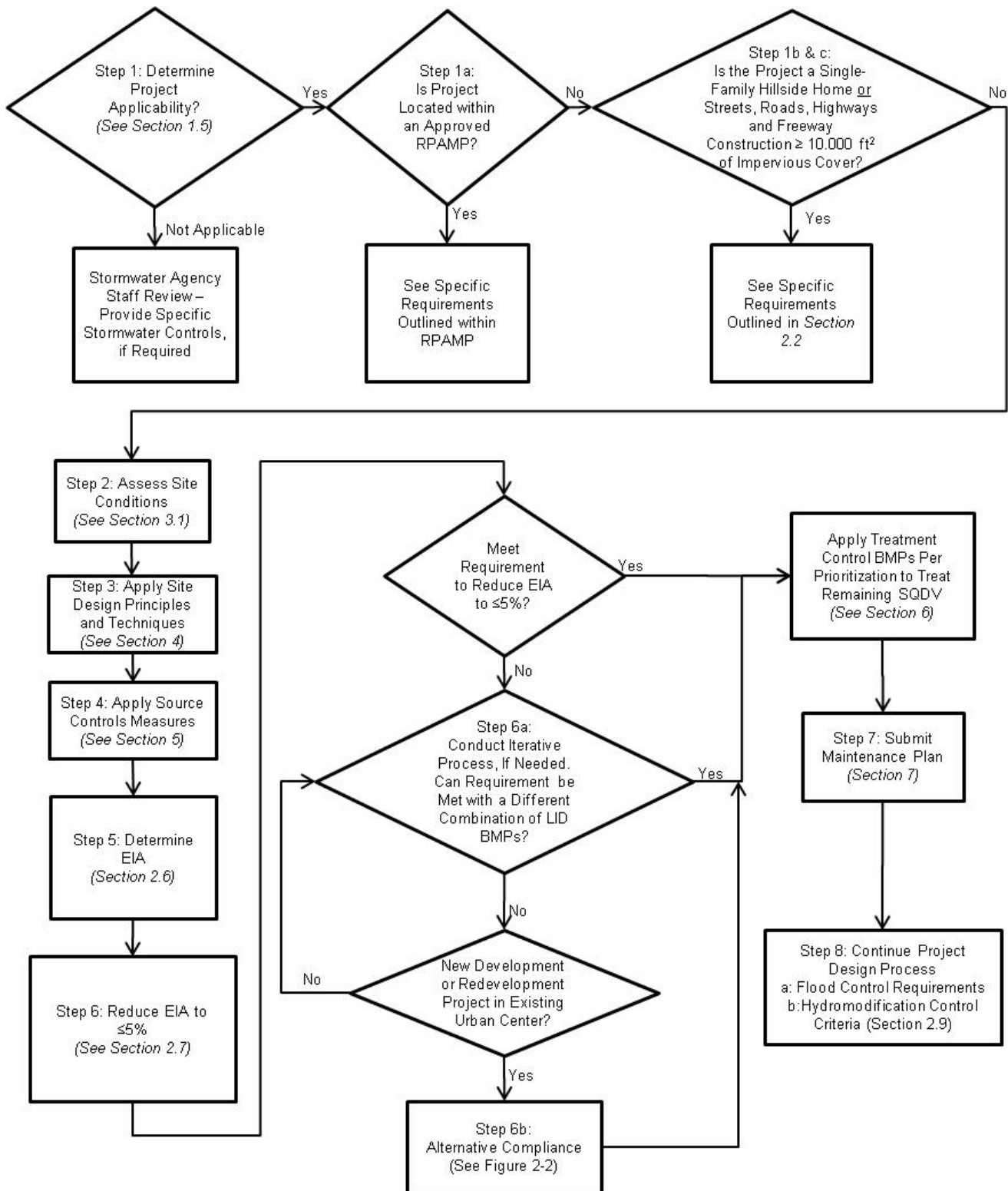
Figure 2-1: Stormwater Management Control Measures Design Decision Flowchart
