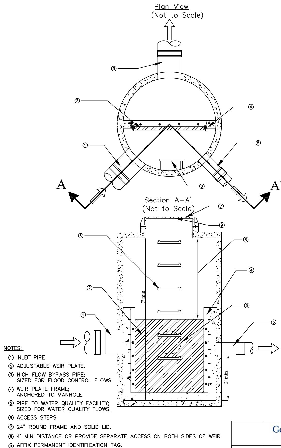
Figure F-1: Flow Splitter Option A
