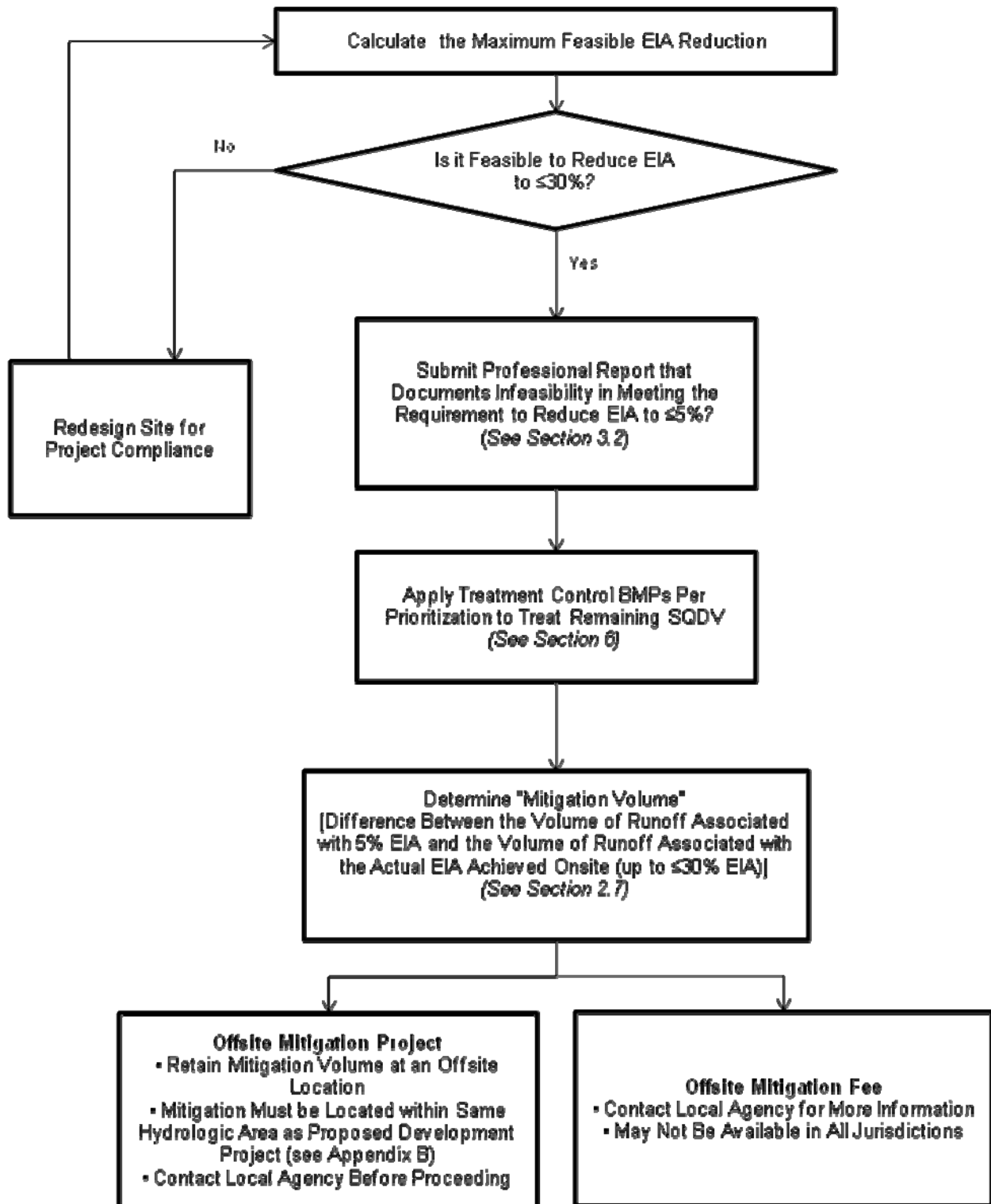
Figure 2-2: Alternative Stormwater Management Control Measures Compliance Decision Flow Chart
