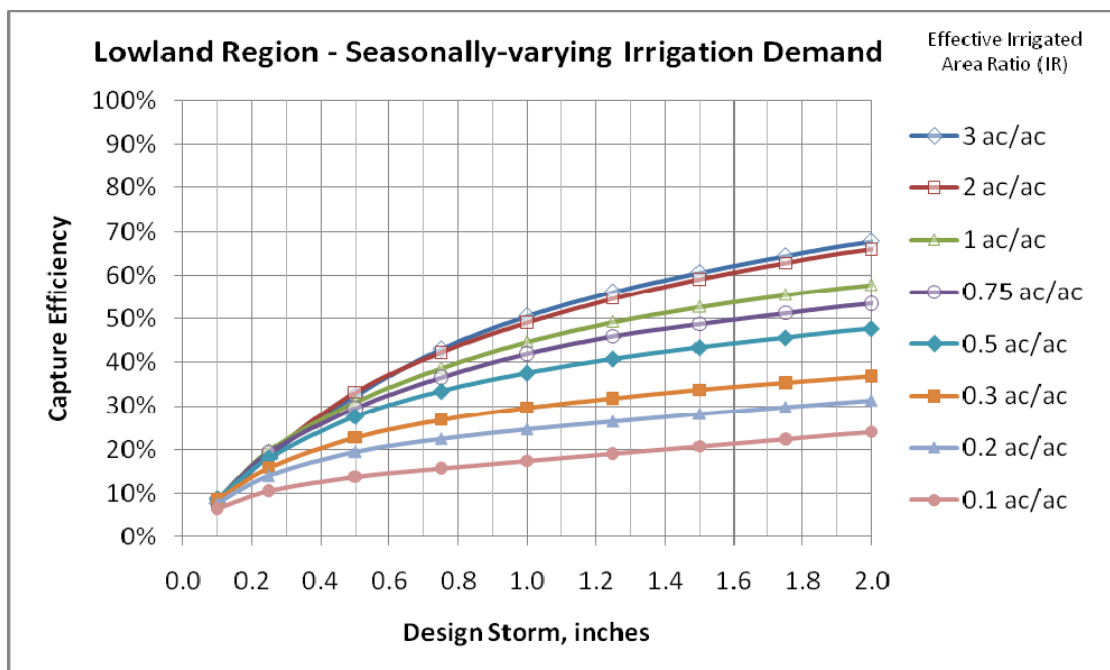
Figure D-3: Percent capture nomograph for systems with seasonally-varying demand in lowland regions of Ventura County
