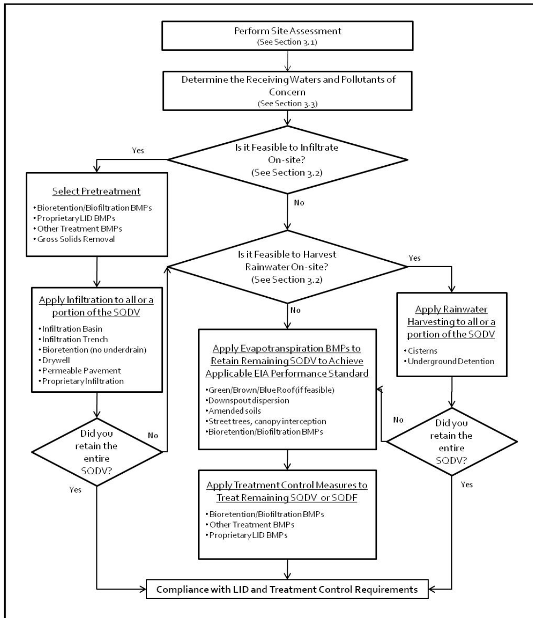
Figure 3-1: LID BMP and Treatment Control Measure Selection Flowchart
