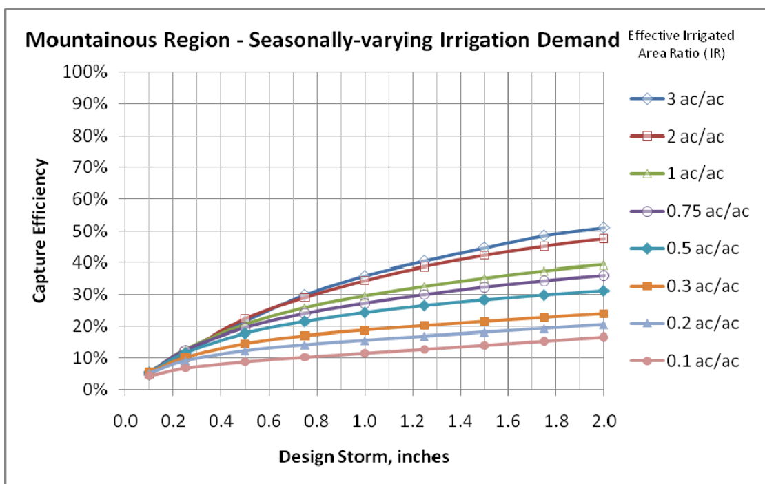
Figure D-4: Percent capture nomograph for systems with seasonally-varying demand in mountainous regions of Ventura County
