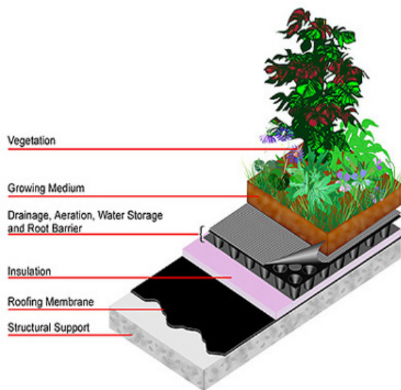
Exhibit B: Green Roof Schematic Courtesy of American Wick
