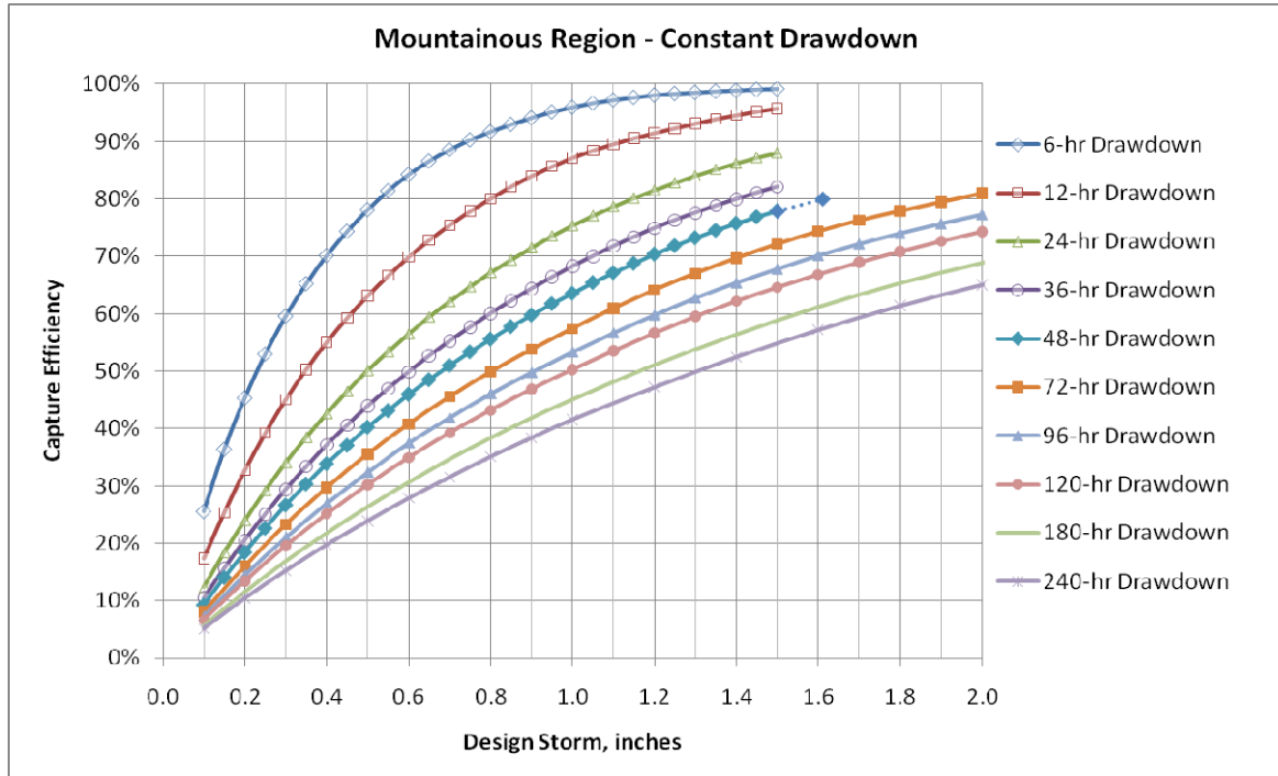
Figure D-2: Percent capture nomograph for systems with constant drawdown in mountainous regions of Ventura County
