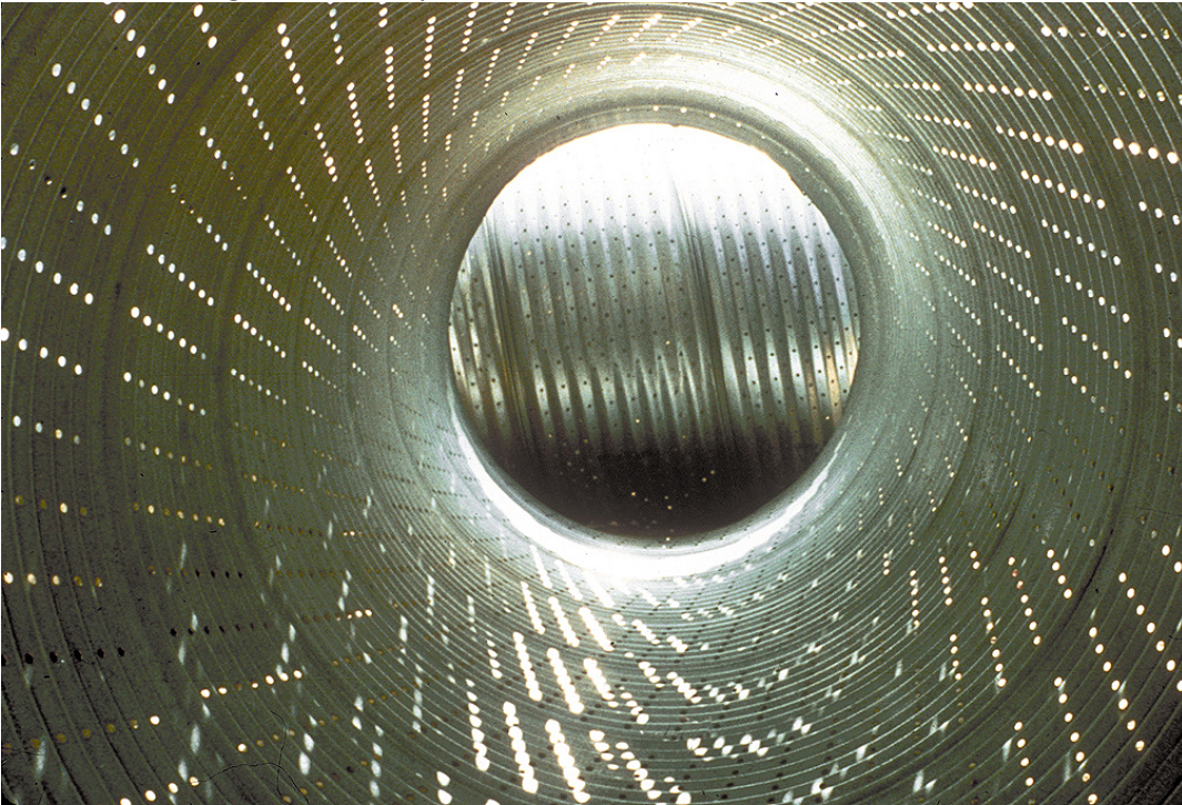
Perforated Corrugated Metal Pipe
