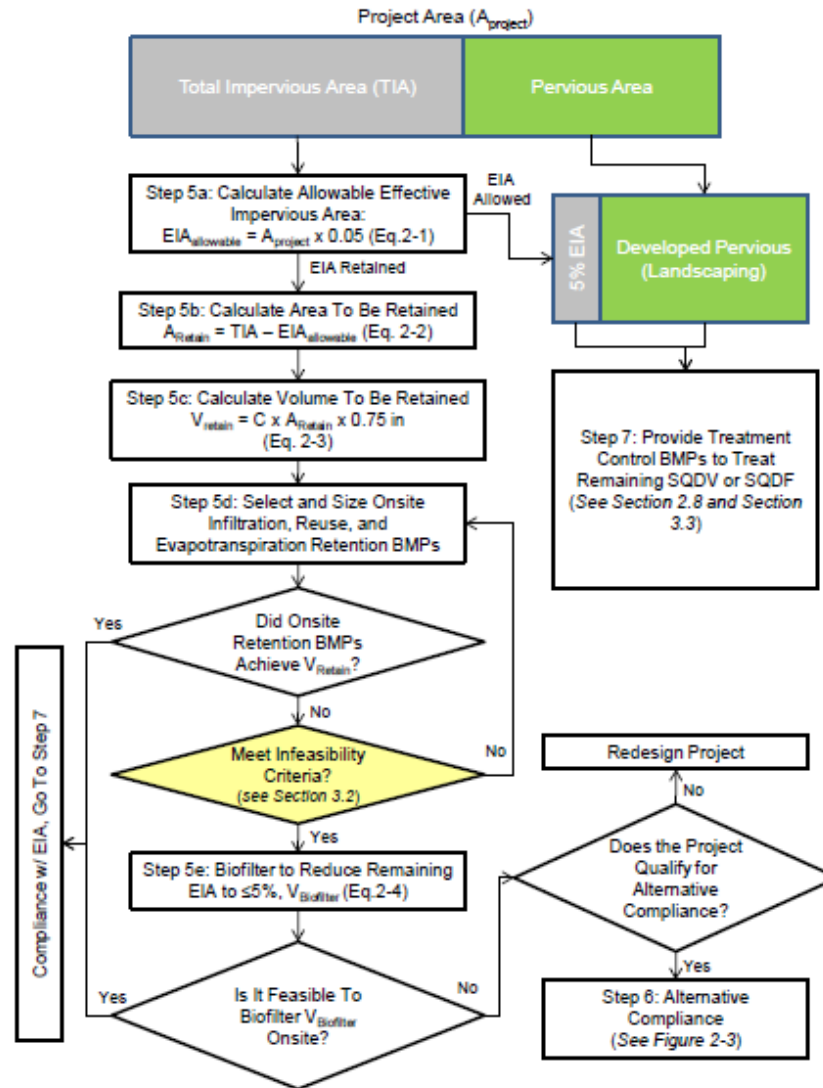
Figure 2-2. Step 5: Apply BMPs to Reduce EIA to \leq 5\%
