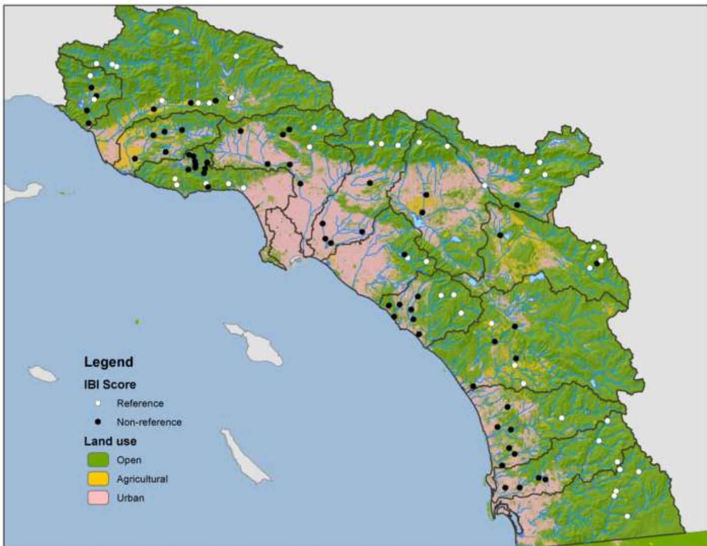
Figure 13. Distribution of IBI scores across the region.
