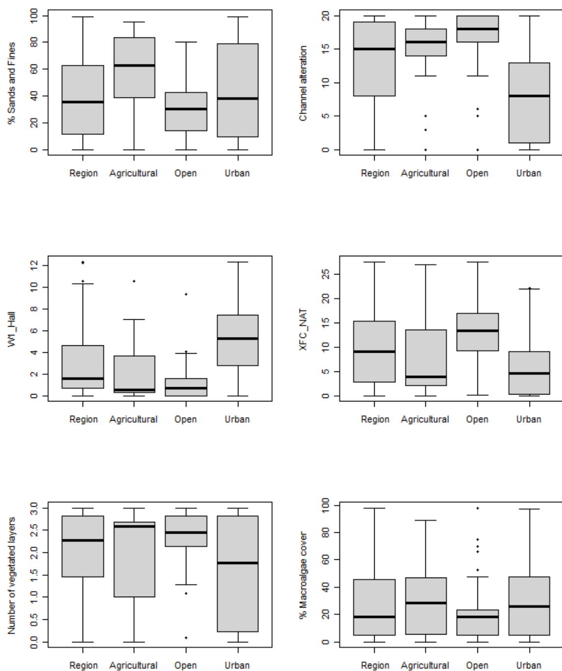
Figure 11. Distribution of % sands and fines, channel alteration, W1_Hall, XFC_NAT, average number of vegetation layers in the riparian zone, and % macroalgae cover, across the region and by land use. X-axes are identical for all panels in the figure.
