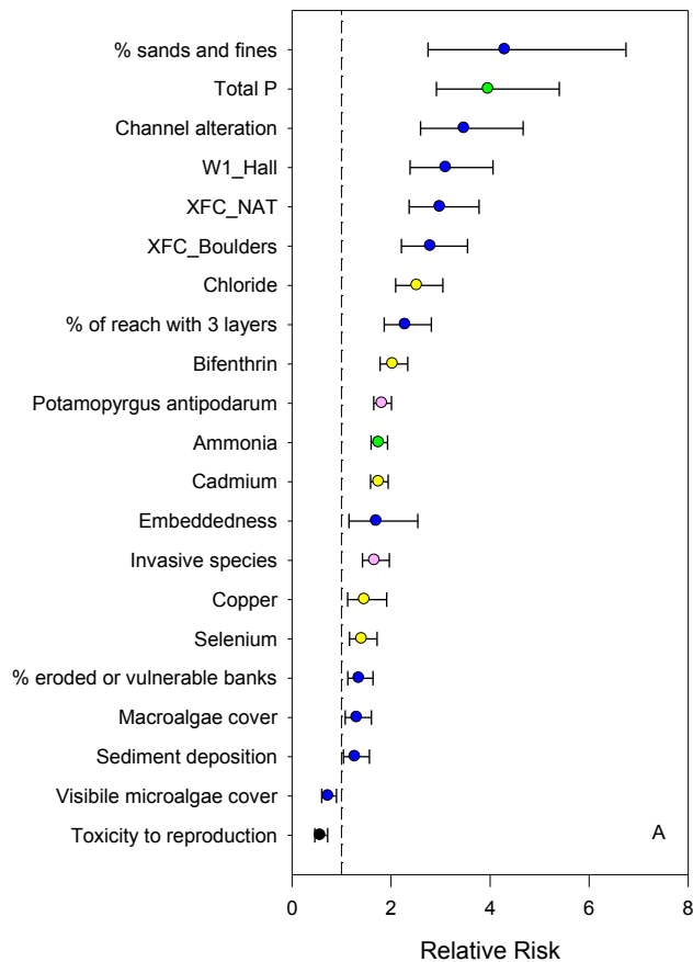
Figure 14. Relative risks of selected stressors for non-reference IBI scores ( \leq 39 ). Physical habitat, water chemistry, and toxicity stressors (A). Blue symbols indicate stressors related to physical habitat. Green symbols indicate stressors related to nutrients. Yellow symbols indicate stressors related to water chemistry. Black symbols indicate stressors related to toxicity. Pink symbols indicate stressors related to biology. GIS stressors. Red symbols indicate metrics related to landcover. Green symbols indicate metrics related to transportation. Black symbols indicate metrics related to census data (B). Blue symbols indicate metrics related to hydrology. Yellow symbols indicate metrics related to mining. White symbols indicate metrics related to grazing. Error bars indicate 95% confidence intervals. The dashed line indicates a relative risk of 1 (i.e., no increased risk from stressor).
