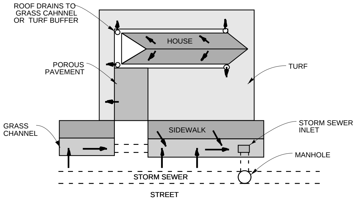
Figure 3-1 EXAMPLES OF MINIMIZING FLOW FROM IMPERVIOUS AREAS
