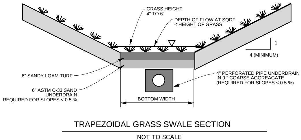
Figure 5-3 GRASS SWALE FILTER
