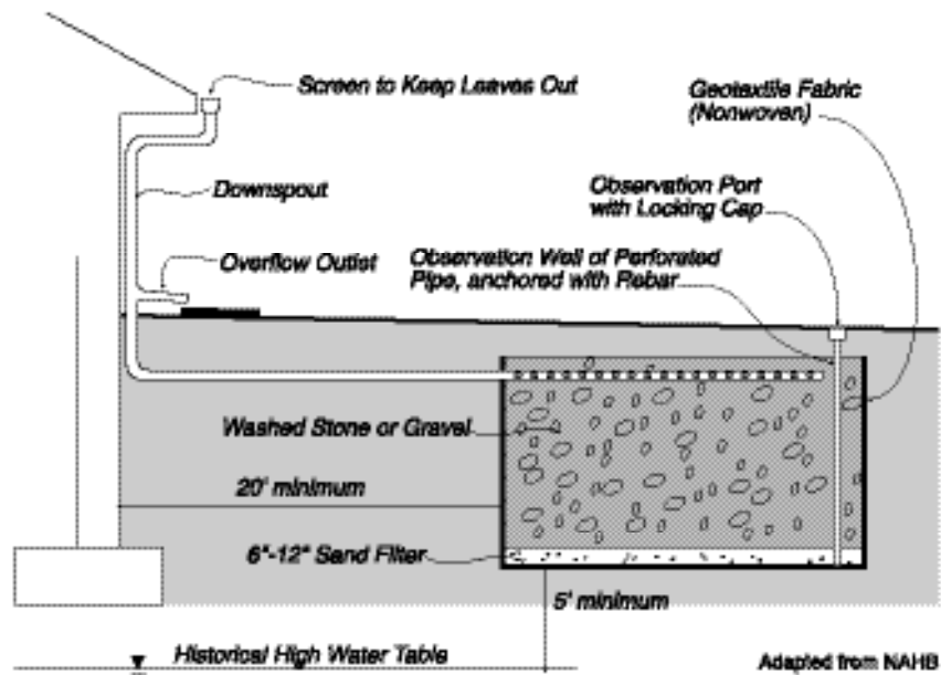
FIGURE 5-16. INFILTRATION VAULT
