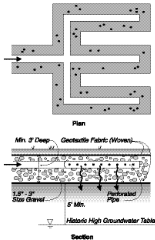
FIGURE 5--17. LEACH FIELD
