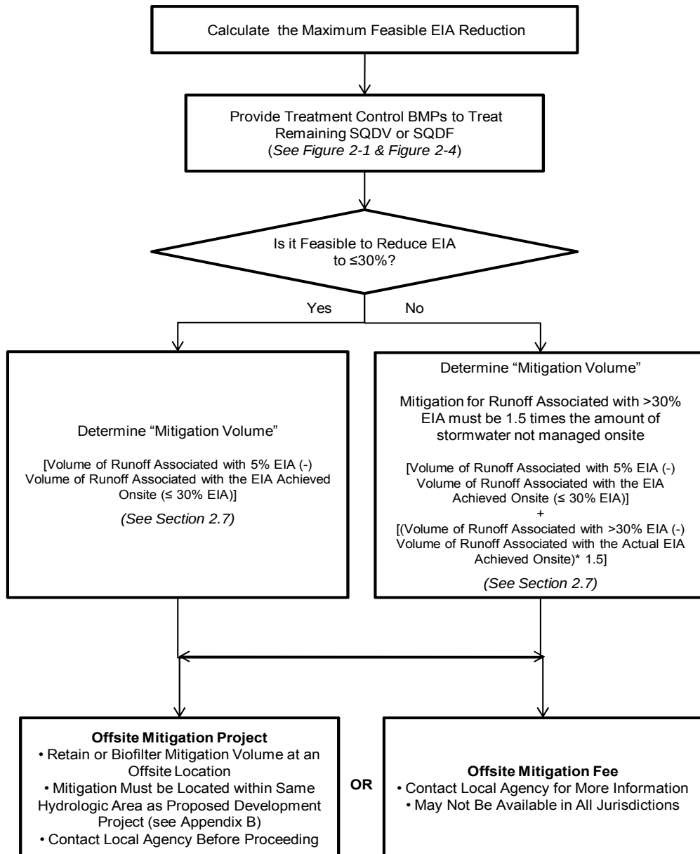
Figure 2-3: Alternative Stormwater Management Control Measures Compliance Decision Flow Chart
