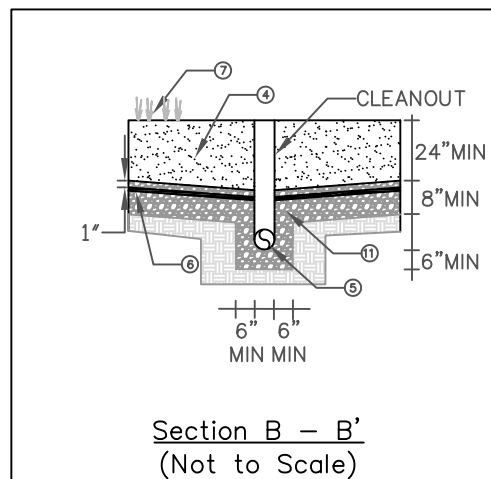
Geosyntec consultants Figure 6-22: Sand Filter
